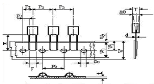
Fig.1 P=5.0、7.5mm
